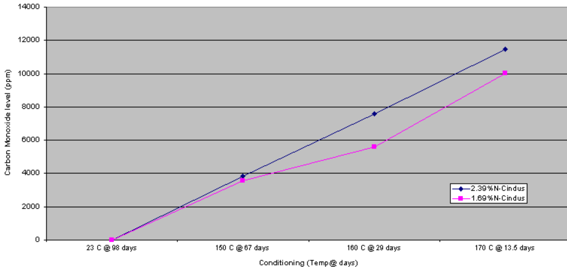
Carbon Monoxide content vs Conditioning parameters.
