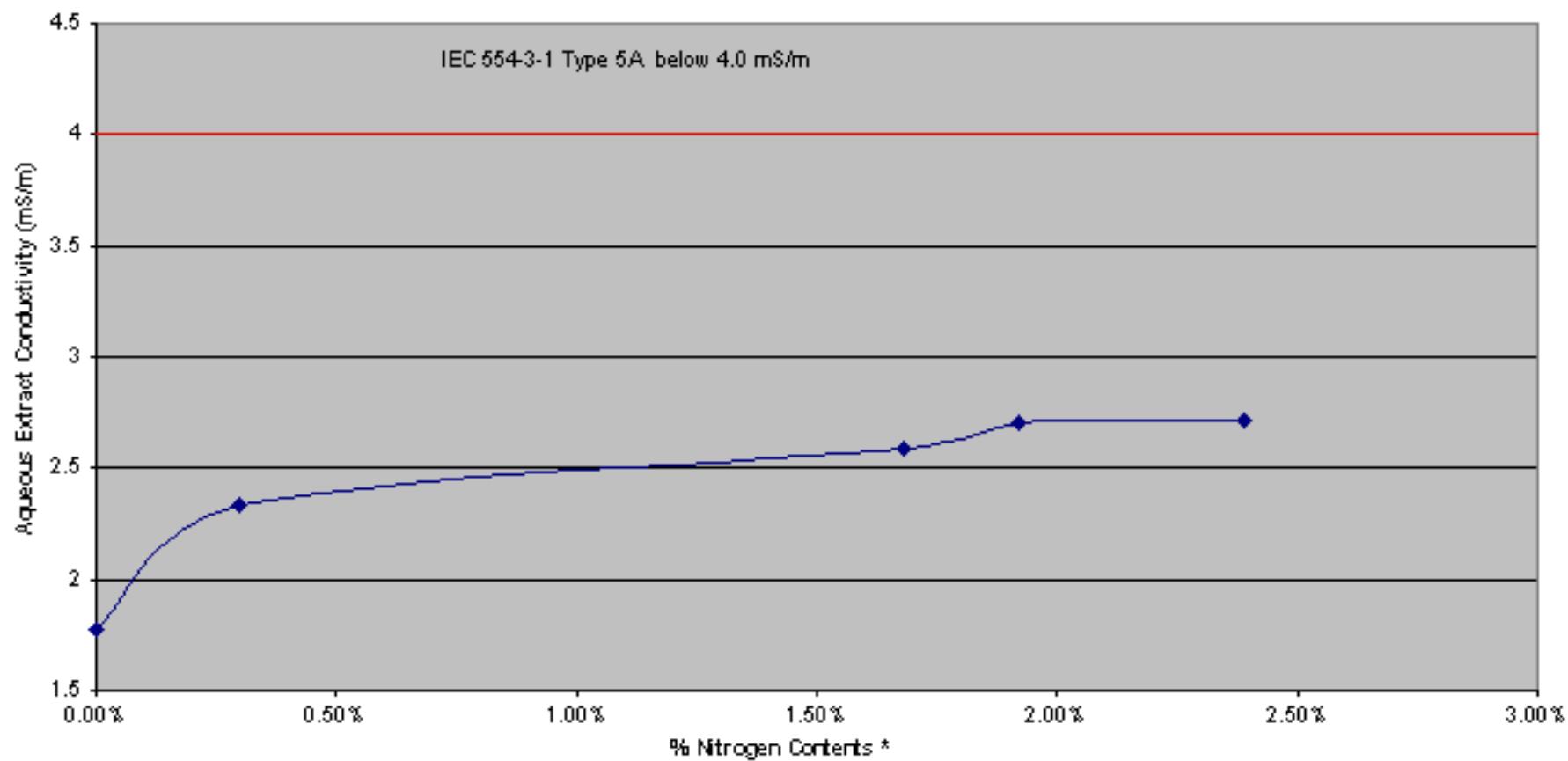
Aqueous Extract Conductivity vs. % Nitrogen
